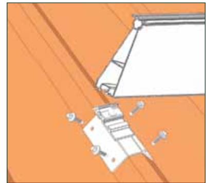
❶ Mounting of the Fix2000ClickTop connector.
